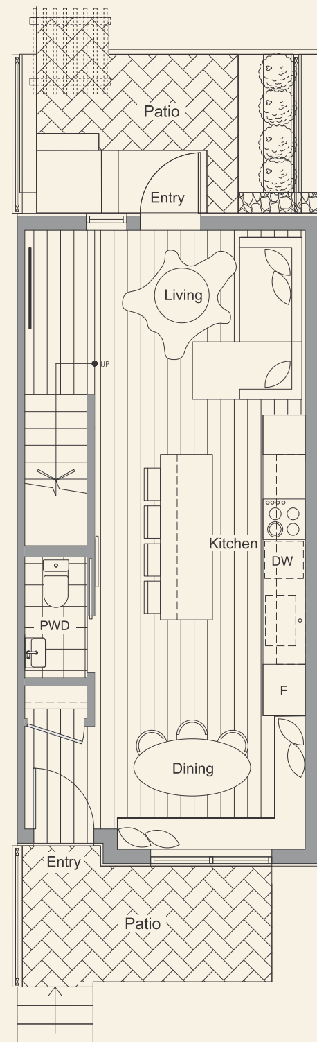
MAIN FLOOR
