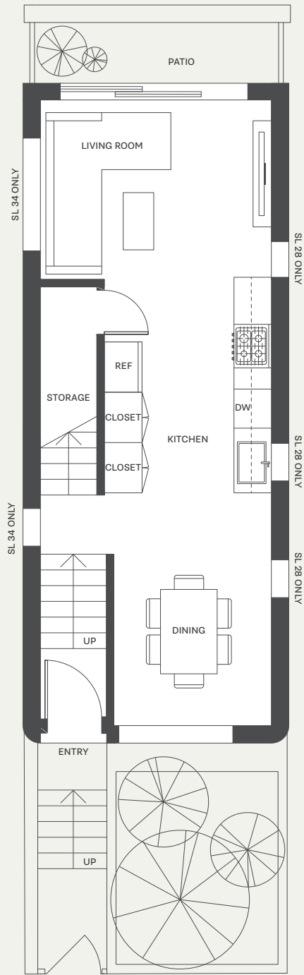
MAIN LEVEL
