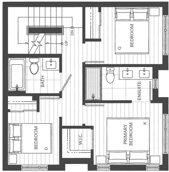
UPPER LEVEL
